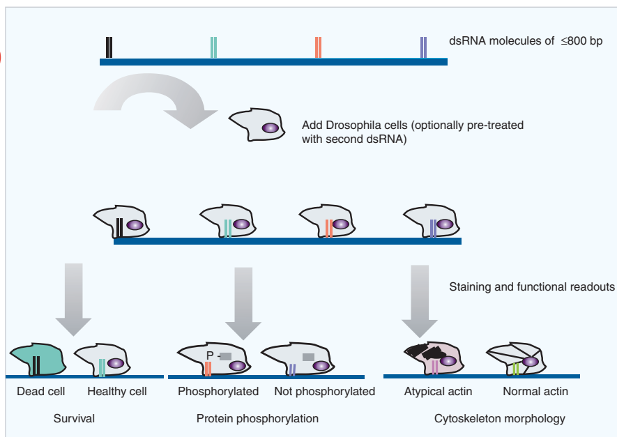
Figure 1 | Schematic of dsRNA microarray for Drosophila cells.
