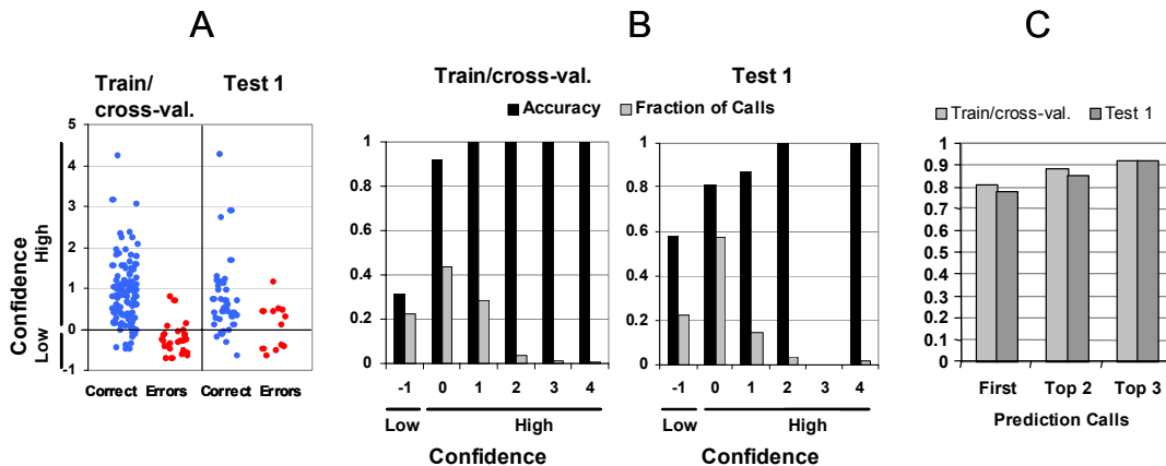
Figure 4. Individual sample errors and confidence calls (A), accuracy bar graphs (B) and performance considering second-and third most confident prediction (C) for the train/cross-validation and test datasets.
