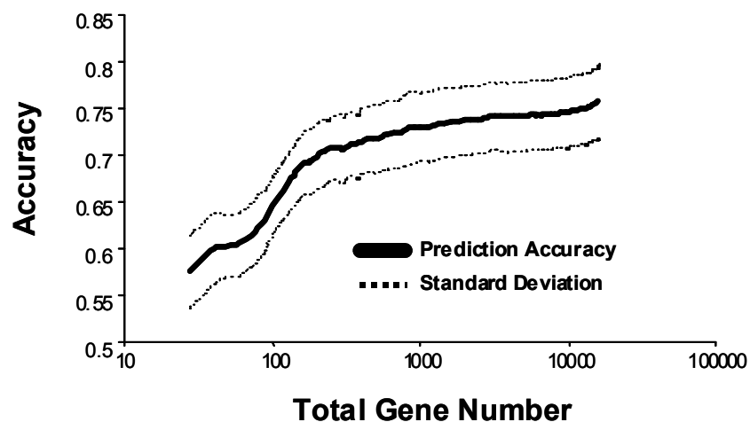
Figure 5. Mean classification accuracy and standard deviation plotted as a function of number of genes used by the classifier. The prediction accuracy decreases with decreasing number of genes.
