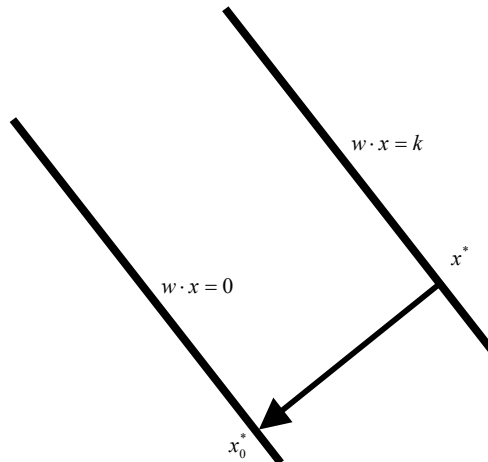
Figure 6. The distance between points x and x_0 .
